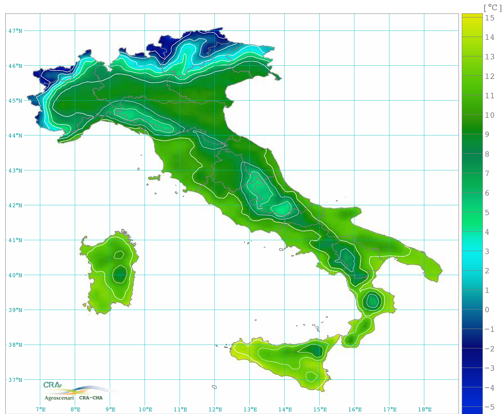
Temperatura minima media annua (1961-1990)
