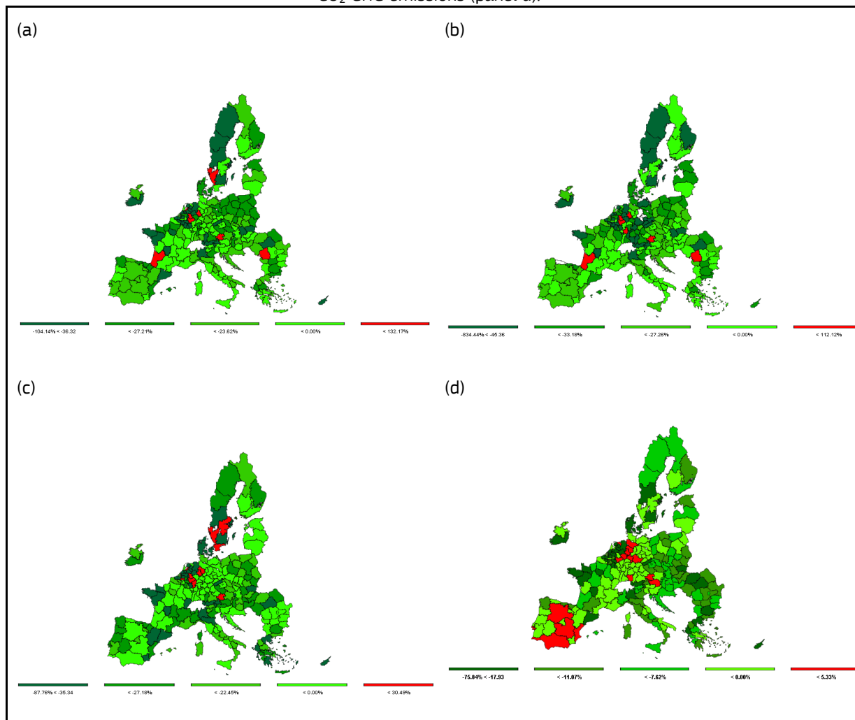
Figure 8. Changes in the F2F and BDS targets and CAP 2014-2020 scenario compared to the baseline (2030) for nitrogen surplus (panel a); nitrogen leaching per hectare (panel b); ammonia emissions (panel c) and non-CO 2 GHG emissions (panel d).
