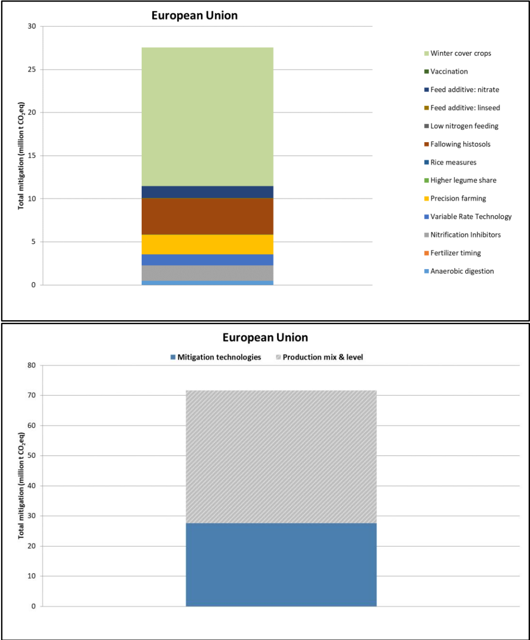
Figure 9. Contribution of each technology and agronomic practice (above) and of production change (below) to total mitigation of non-CO2 and CO2 emissions under the F2F and BDS targets and CAP 2014-2020 scenario
