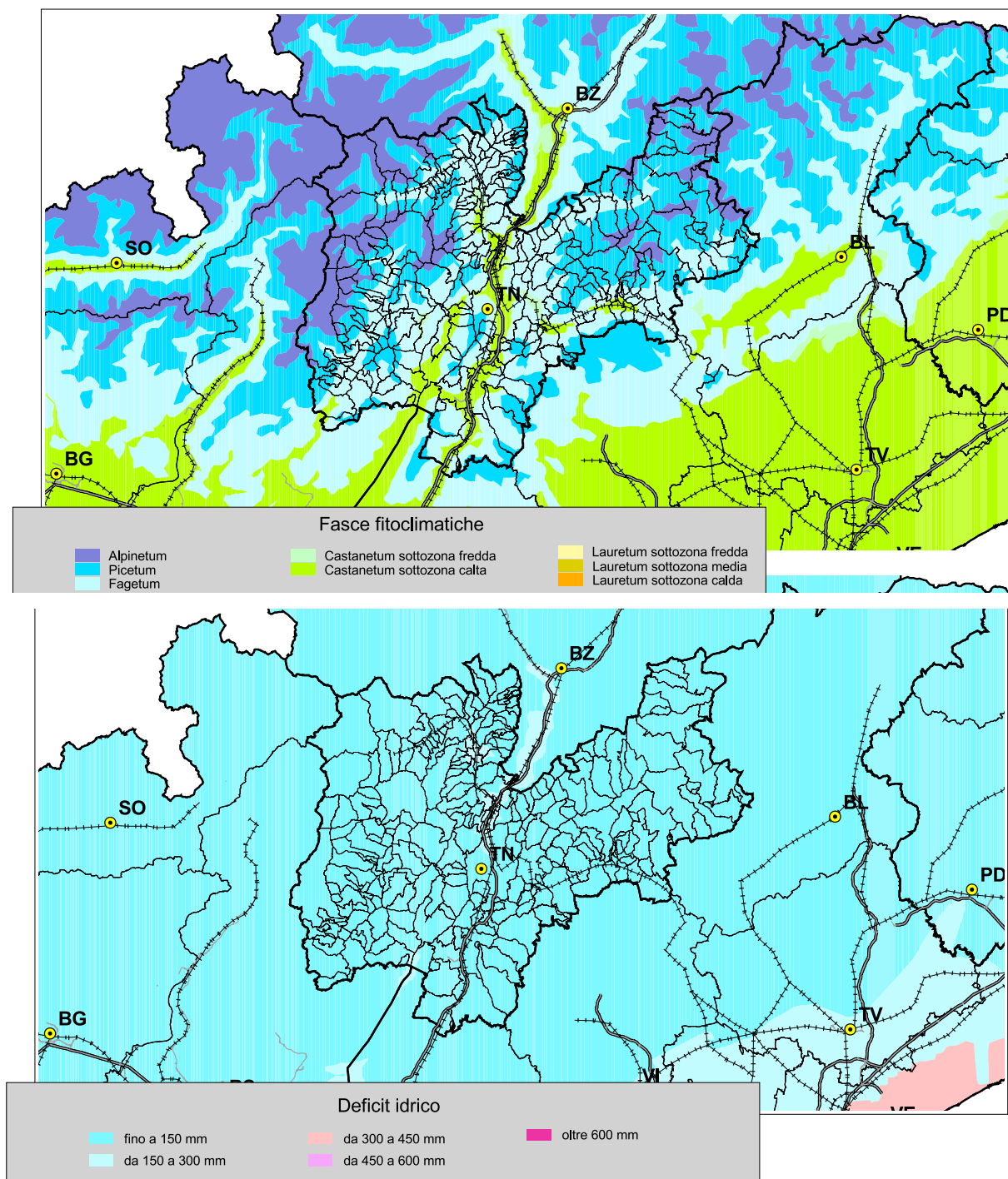
fig. 3d - Clima
