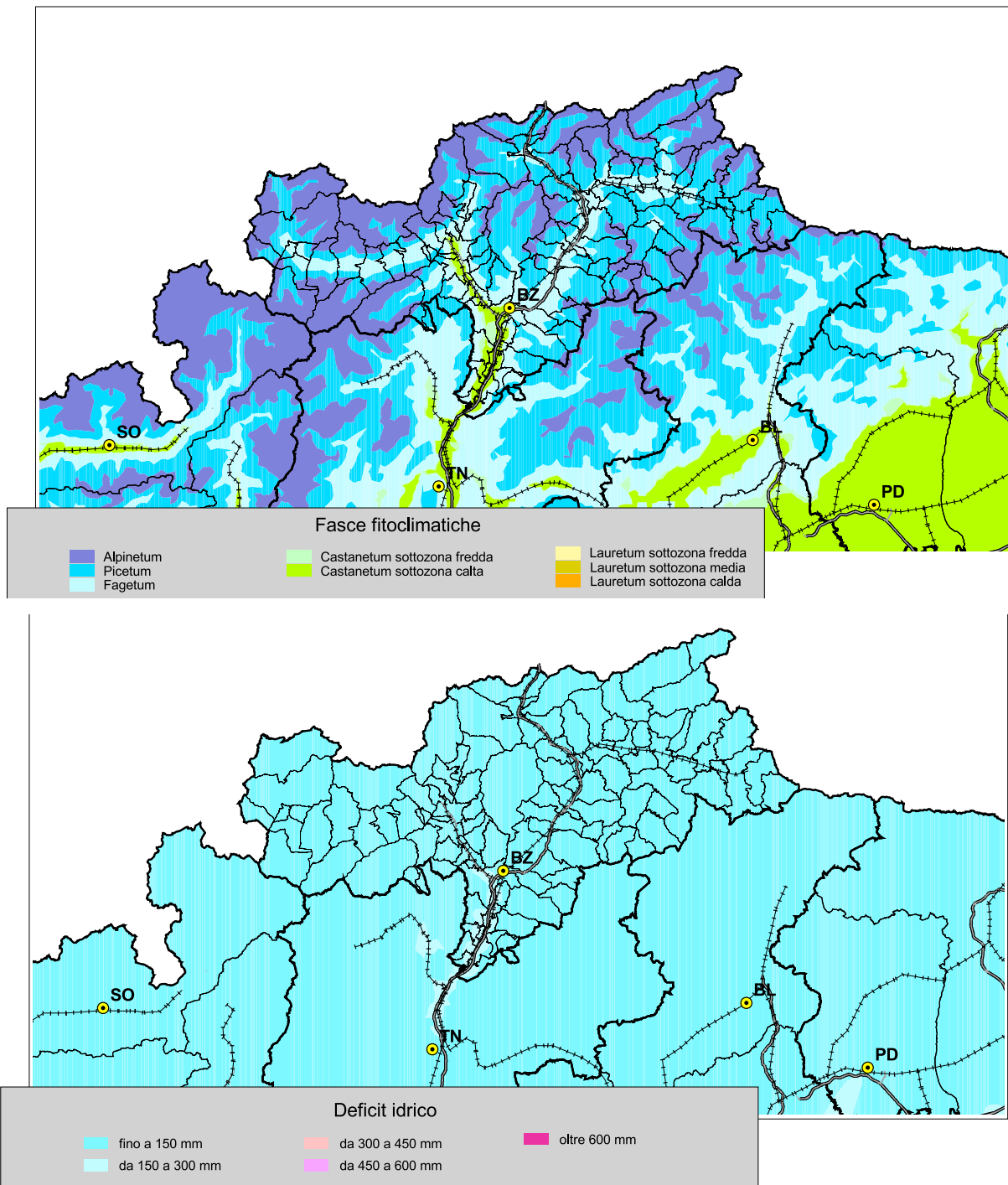
fig. 3d - Clima
